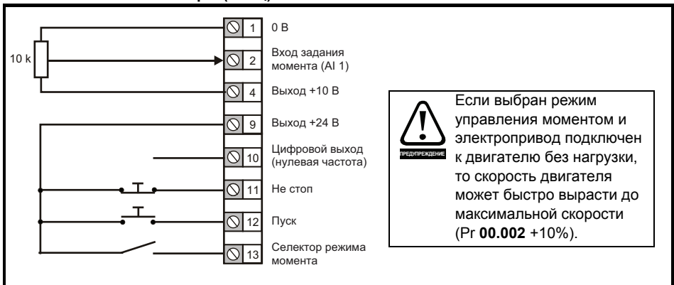
Рис. 4-14 Pr 00.005 = Torque (60 Гц)
