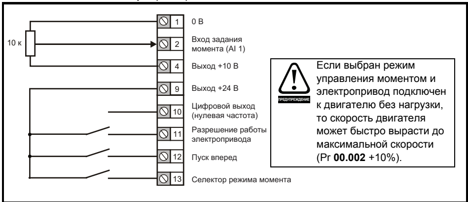
Рис. 4-13 Pr 00.005 = Torque (50 Гц)
